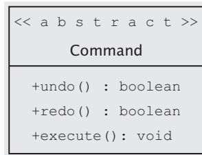
Figure 11.16 The command class
