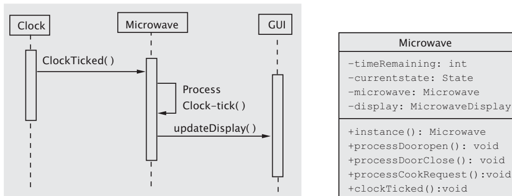
Figure 10.5 Sequence diagram for processing a clock tick Figure 10.6 Microwave class diagram
