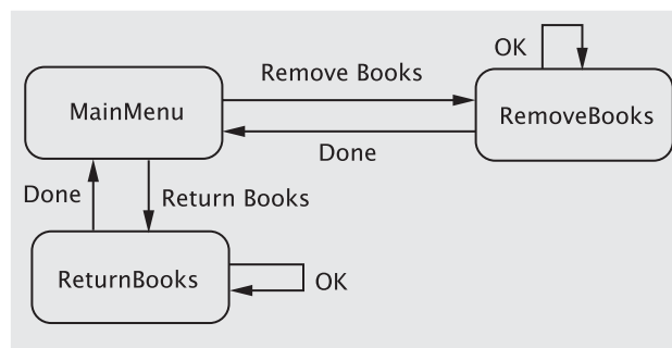
Figure 10.26 Remove books and return books
