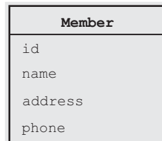
Figure 6.3 UML diagram for the class Member
