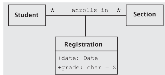
Figure 3.4 Using an association class
