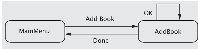
Figure 10.23 Main menu and add books
