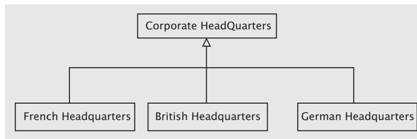
Figure 5.2 Singleton hierarchy
