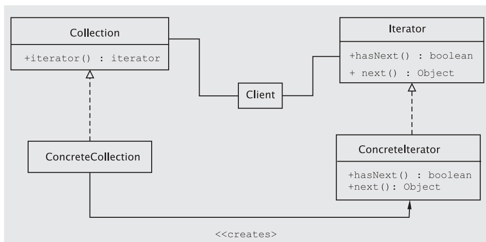
Figure 5.1 Iterator structure
