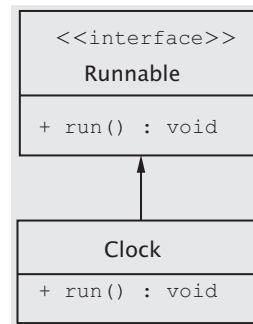
Figure 10.8 Clock
