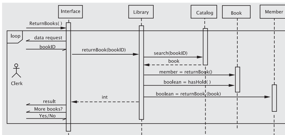
Figure 7.4 Sequence diagram for returning books
