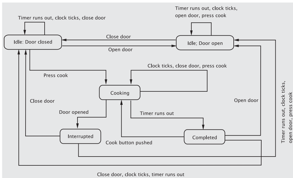
Figure 10.2 State transition diagram for the microwave oven
