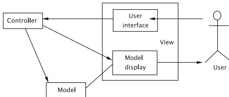
Figure 11.2 An alternate view of the MVC architecture
