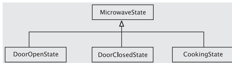
Figure 10.10 MicrowaveState hierarchy
