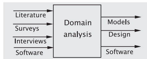
Figure 6.10 Domain analysis
