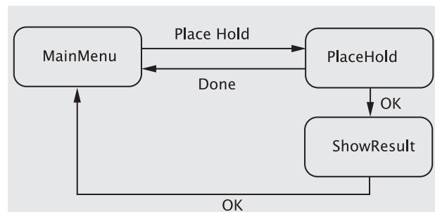
Figure 10.27 Place hold
