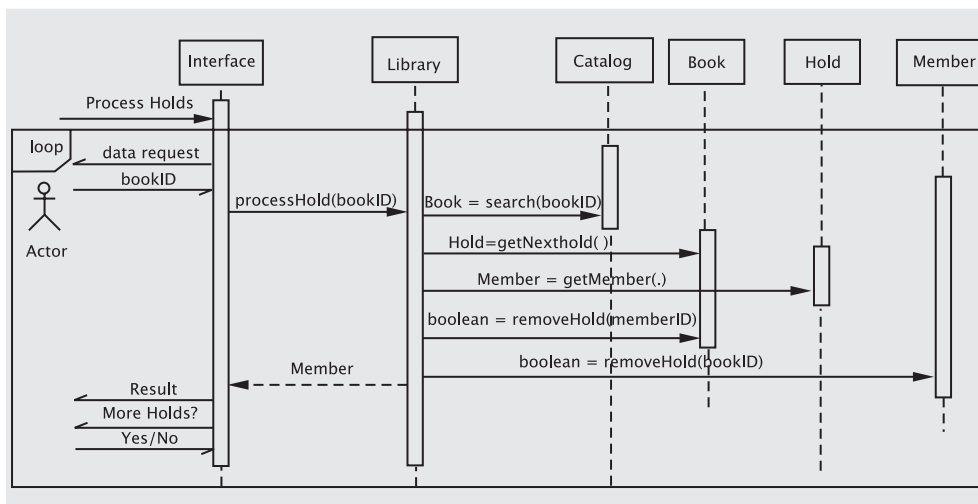
Figure 7.8 Sequence diagram for processing holds
